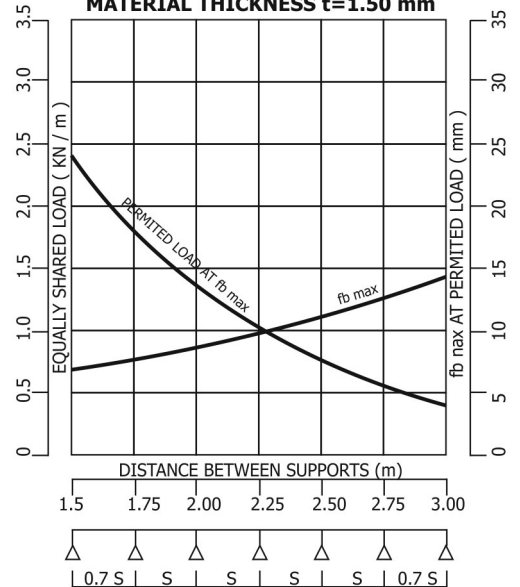
CABLE TRAY H:60 LOADING DIAGRAM MATERIAL THICKNESS t=1.50 mm
